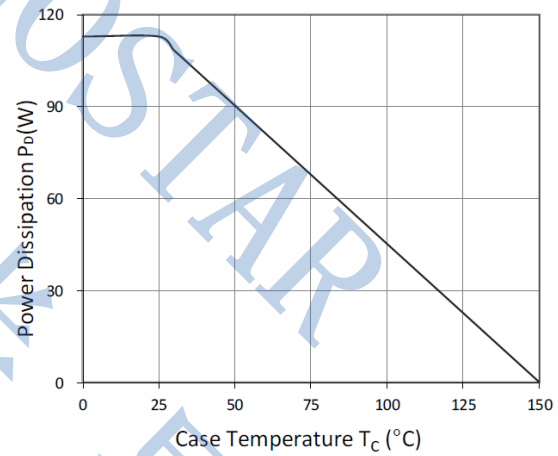
Figure 10. Power Dissipation
