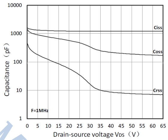
Figure 8. Capacitance Characteristics
